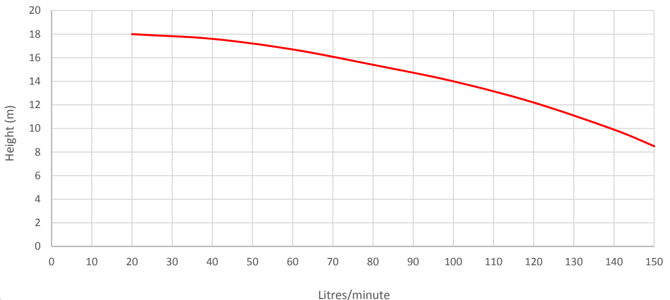
Pump Performance
