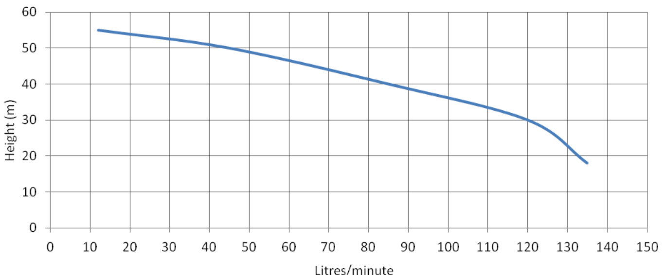
Pump Performance
